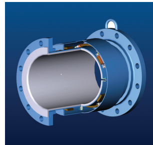
Fully welded coil housing
